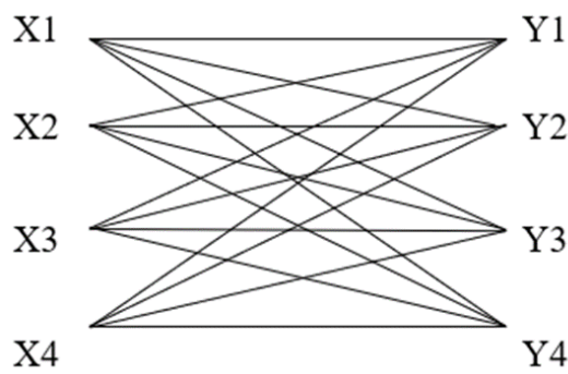
Figure 1. The graph of fuzzy relationships
